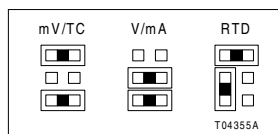
Figure C-2. IMASI23 Six Pin Jumper Block Configuration
